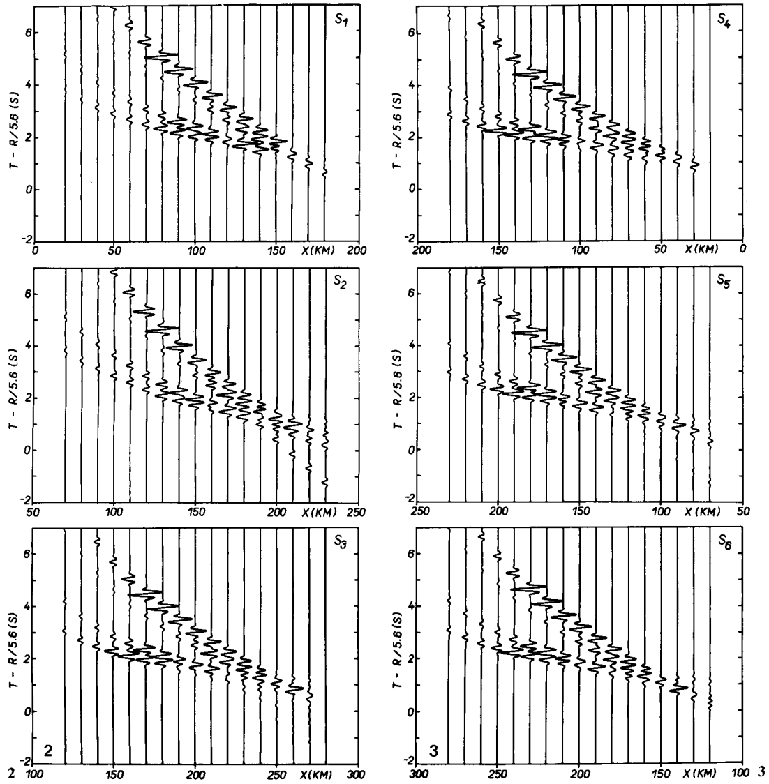
Fig. 2. Ray theoretical seismograms for the model of laterally varying Earth's crust shown in Fig. 1, for sources S_1 (top figure), S_2 (middle figure), S_3 (lower figure). The epicentral distance is denoted by R , the distance along the profile by x . Reduction velocity equals 5.6 km/s
