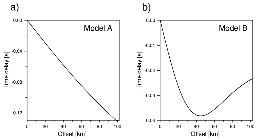
Figure 4. Differences in traveltimes of waves propagating in the attenuating medium and in the elastic background. (a) traveltimes differences in model A and (b) traveltimes differences in model B.
