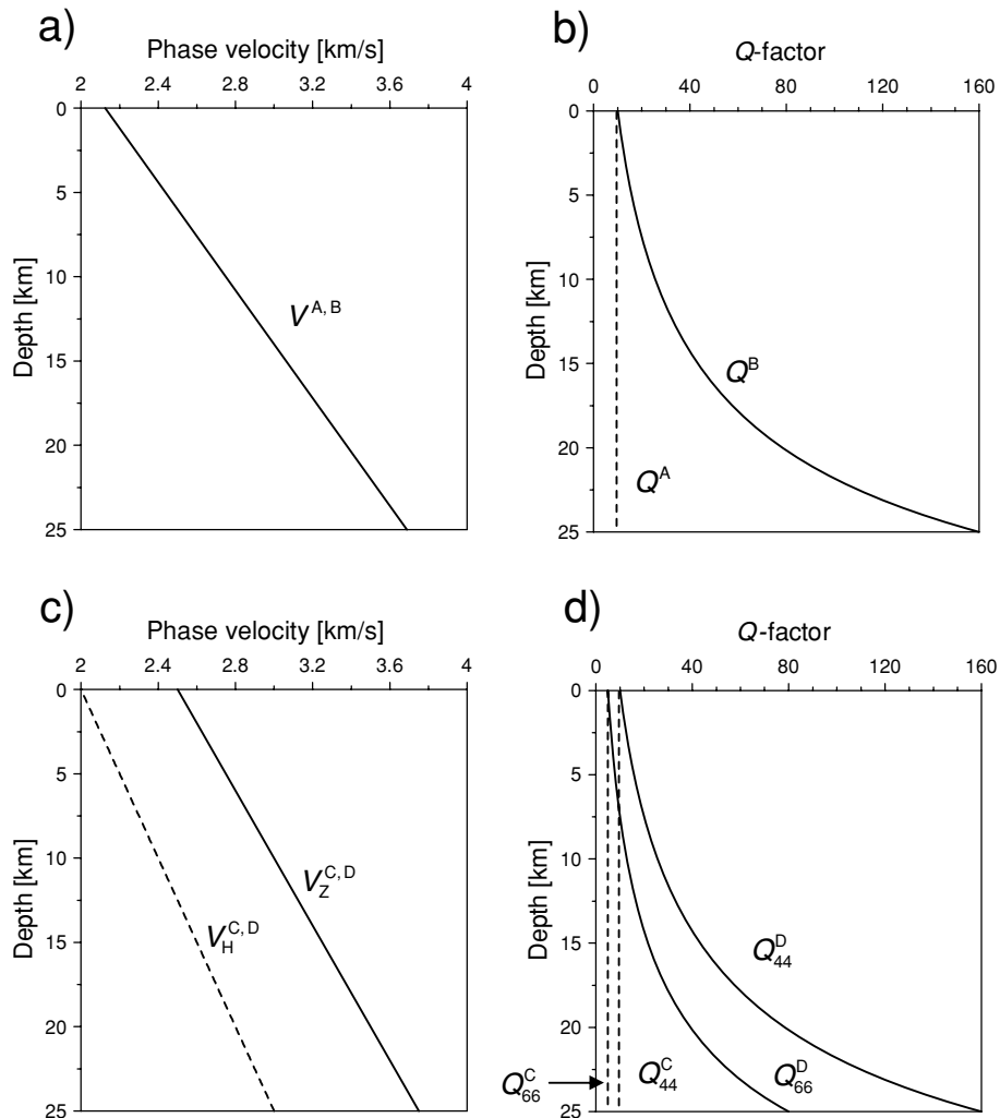
Figure 2. SH phase velocities and Q -factors as a function of depth. (a) Phase velocity in the elastic background of models A and B, (b) Q -factors for model A (dashed line) and model B (solid line), (c) phase velocity in the elastic background of models C and D and (d) Q -factors for model C (dashed line) and model D (solid line). V_H , the horizontal phase velocity and V_Z , the vertical phase velocity.
