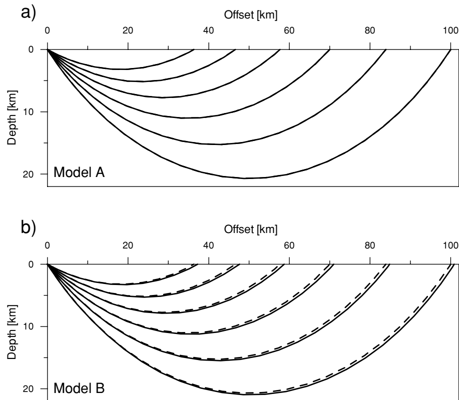
Figure 3. Ray fields in models A (a) and B (b). Solid line, rays calculated in the viscoelastic medium; dashed line, rays calculated in the elastic background. For parameters of the media and rays, see the text.
