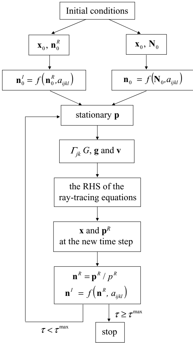
Figure 1. A scheme of the numerical procedure for ray tracing in anisotropic viscoelastic media.
